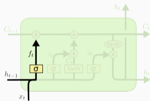
Figure 5: 遗忘门
